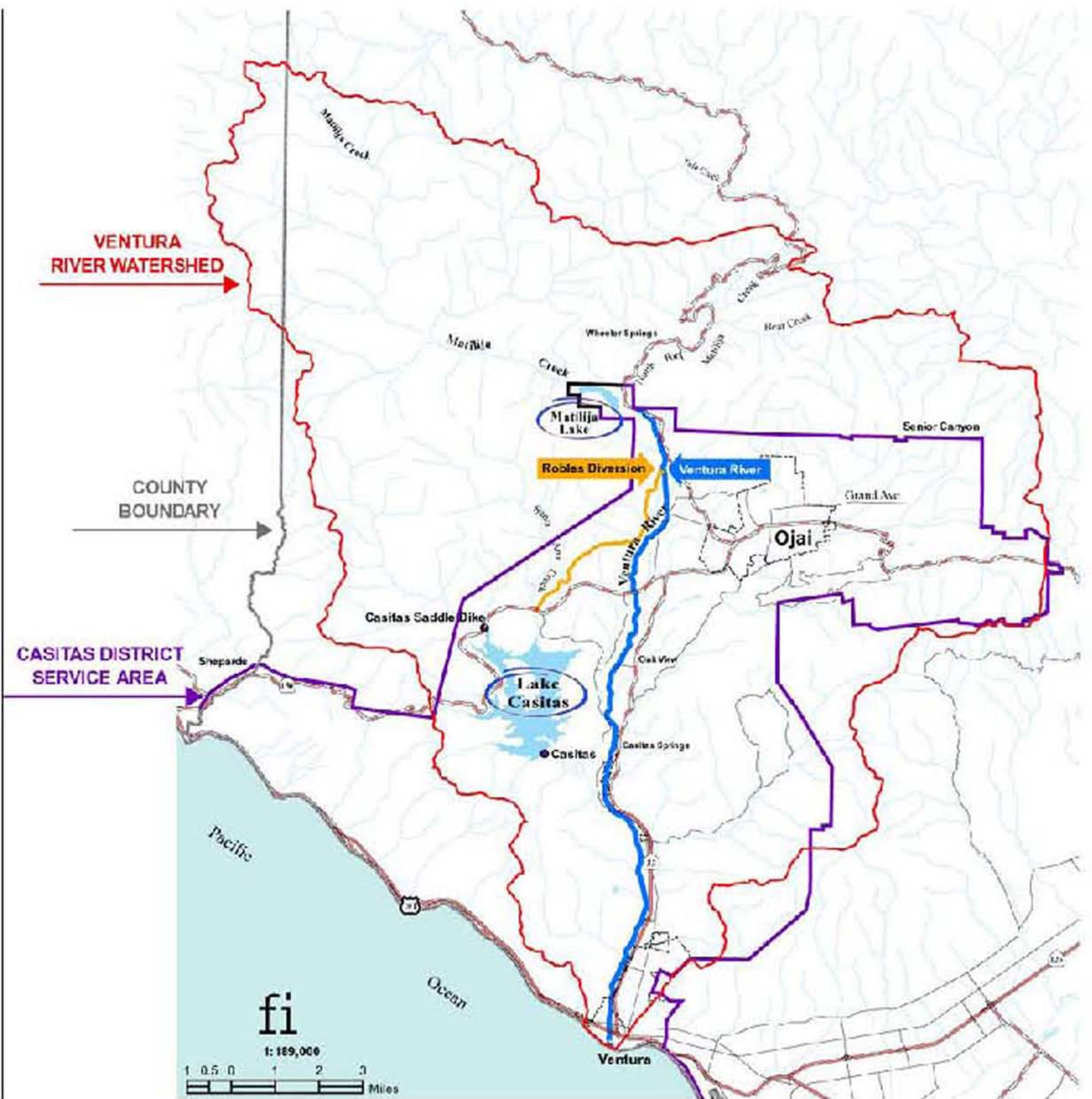
Figure 3-10b Casitas Municipal Water District Major Infrastructure WCVC IRWM Region
